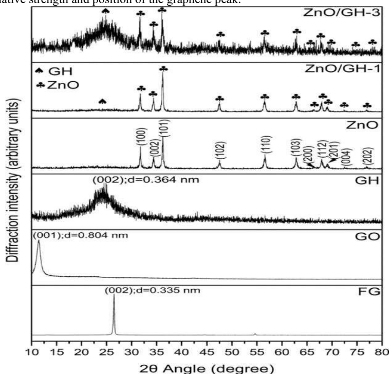
Graph -1 XRD patterns of FG, GO, GH, ZnO, and ZnO/graphene nanocomposites.
