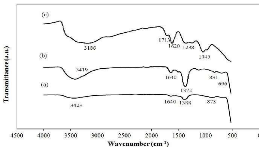
Graph -1 FTIR spectra of (a) ZnO, (b) ZnO/rGO and (c) GO.
