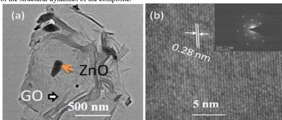
Fig. - 5 TEM image of graphene-ZnO nanocomposites
